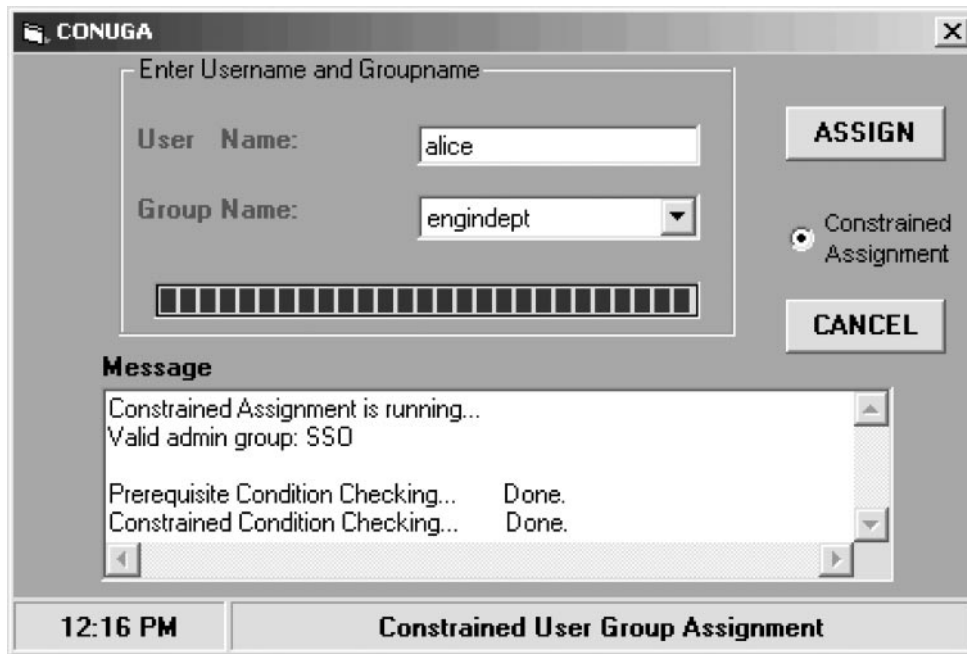
Figure 7. CONUGA interface.
