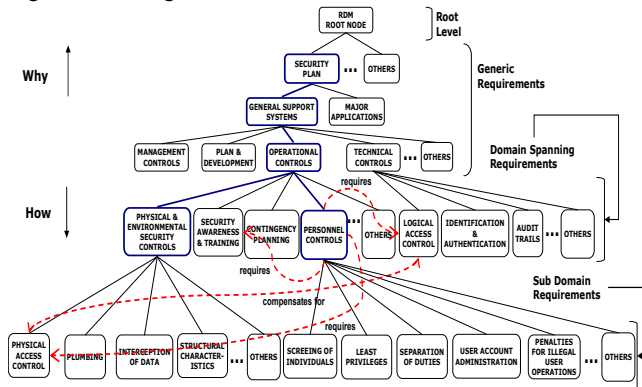
Figure 2: Partial Security Requirements Category Hierarchy
