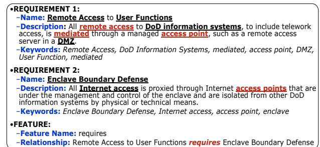
Figure 5: Identifying dependencies using Keywords
