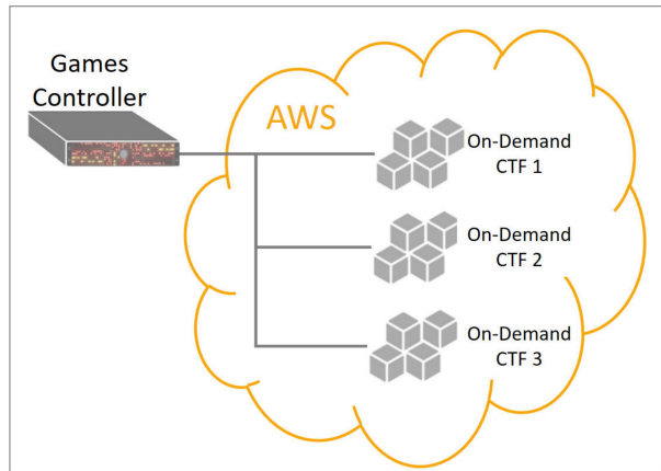
Figure 1: CTF-as-a-Service Overview.
